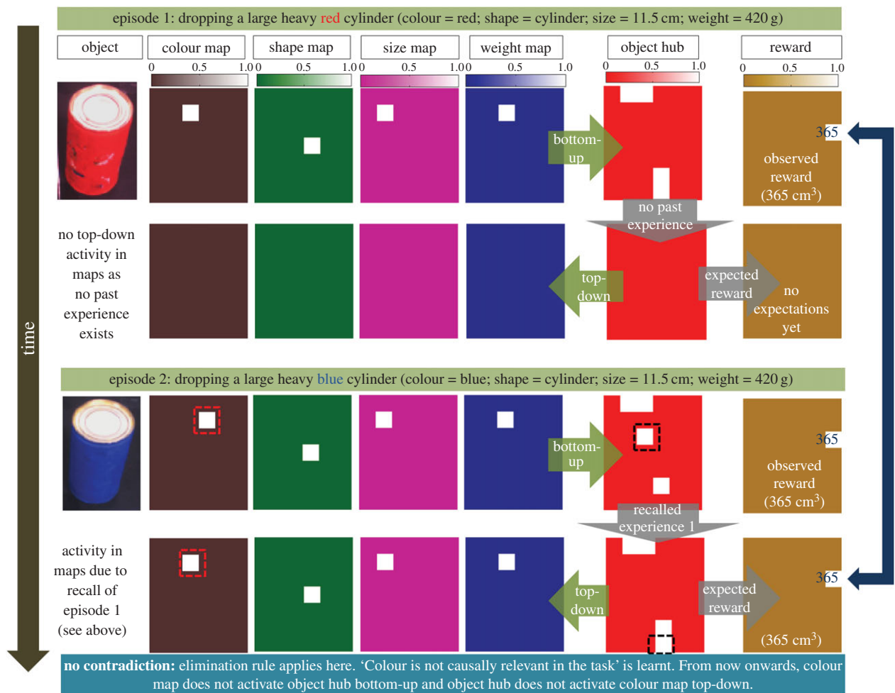
Figure 6. Abstracting colour is an irrelevant property in the Aesop's Fable task. The figure shows neural activity in various property-specific maps, the object hub and the reward hub for a consecutive sequence of two experiences the robot gains by interacting with two similar objects of different colour. In each episode, the first row represents the object and the bottom-up activity of all the neural maps and hubs related to sensorimotor information of the object whereas the second row depicts top-down activity in the maps and hubs due to recalled past episodes. The winning neurons in each network are shown in white (see activity scales on top of the figure). In episode 1, the bottom-up activity (1st row) does not recall any past experience; hence there is no top-down activity (2nd row). The bottom-up activity in the object hub and the reward hub during episode 1 is finally encoded into episodic memory. In episode 2, colour of the object is different from the one explored in episode 1. Upon sensing the new object, the system recalls the experience of episode 1, infers the reward based on it and acts. No contradiction in expected and observed results is found even though there was change in colour property. Elimination rule applies to colour property; the robot learns that the colour of objects is irrelevant to the task. From now on, the object hub and the colour map will not activate each other during any bottom-up or top-down information flow.
